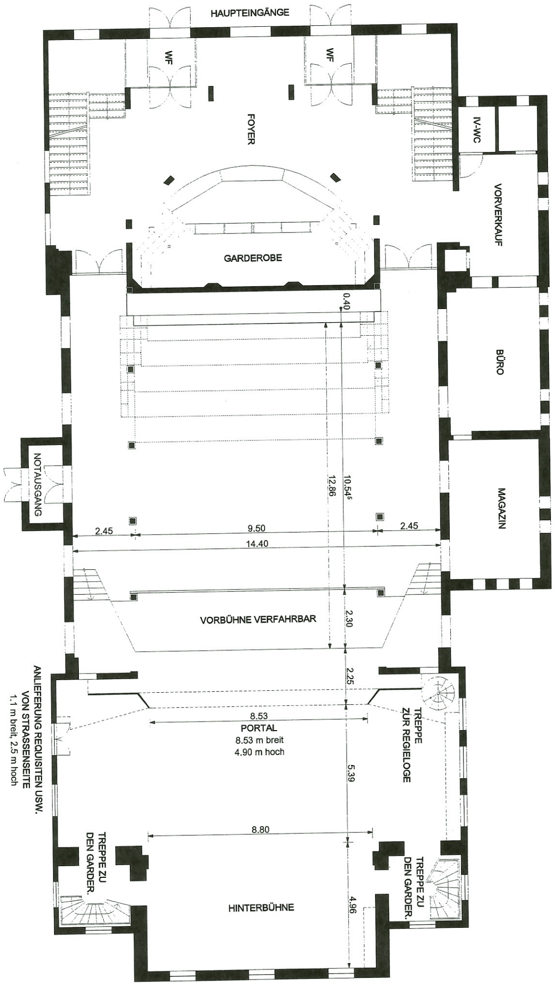
Tonhalle Wil "Theatersaal" 1:100
